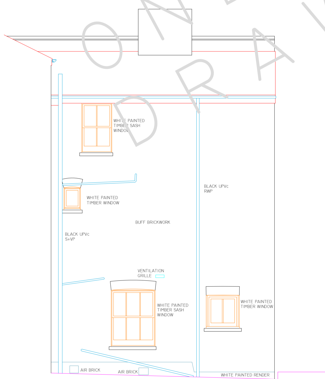
SOUTH ELEVATION 1:50 SCALE
