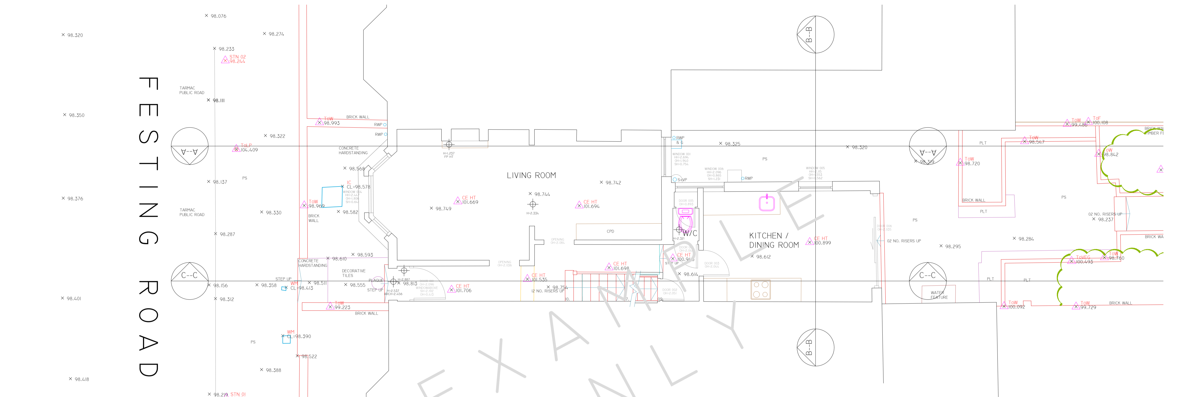
GROUND FLOOR 1:50 SCALE
